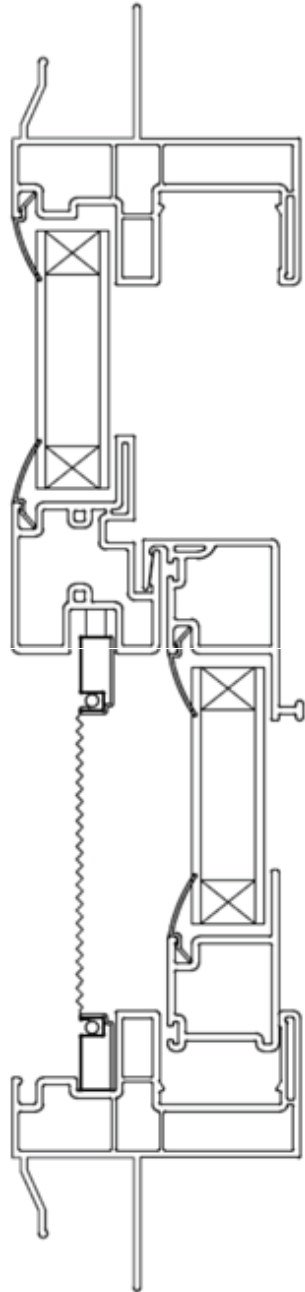
J-CHANNEL FRAME
