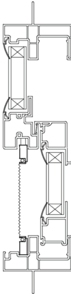
FIN-ONLY FRAME
